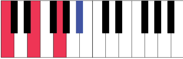
C7
