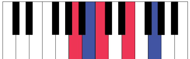
Am9
