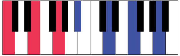
C13
